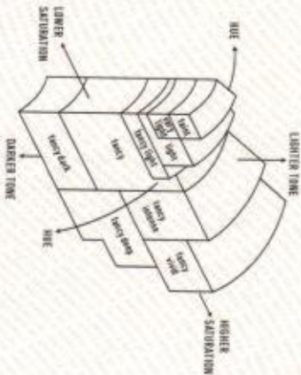
Illustration of GIA fancy color grade interrelationships
